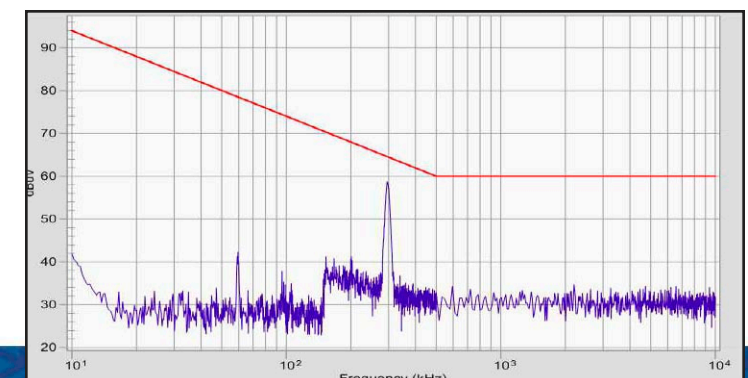
MIL-STD-461E CE102 50 Volt Boost, 3.7A Load (Resistive), HDF-22 EMI Filter
