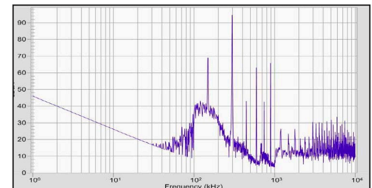
OUTPUT COMMON MODE SPECTRUM 50 Volt Boost, 3.7A Load (Resistive), HDF-22 EMI Filter, 2200μf Output Cap
