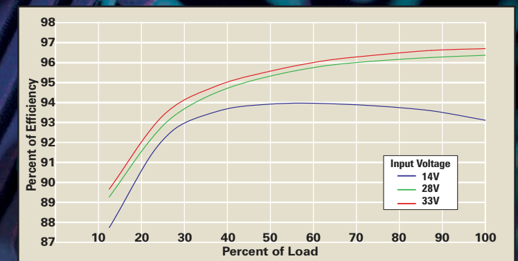
EFFICIENCY VS. LOAD Output at 25°C
