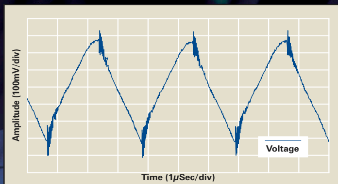
OUTPUT RIPPLE 50 Volt Output, Full Load, 25°C
