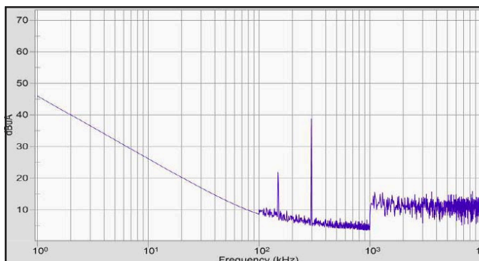
INPUT COMMON MODE SPECTRUM 50 Volt Boost, 3.7A Load (Resistive), HDF-22 EMI Filter, 2200μf Output Cap
