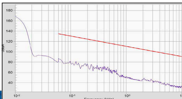
MIL-STD-461E CE101 50 Volt Boost, 3.7A Load (Resistive), HDF-22 EMI Filter
