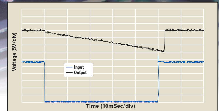
HOLD UP 50V Boost, 3.7A Load, 1600μf Output Cap, 25°C
