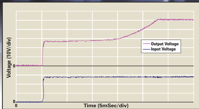
TURN ON TIME 50 Volt Output, 3.7A Load, 25°C
