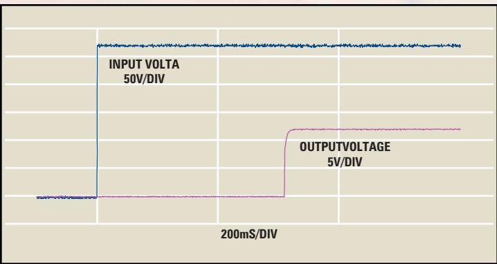
5V HDM+ TURN-ON TIME FROM APPLIED VOLTAGE
