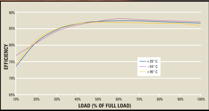
EFFICIENCY VS TEMPERATURE @ NOMINAL LINE 12V HDM+
