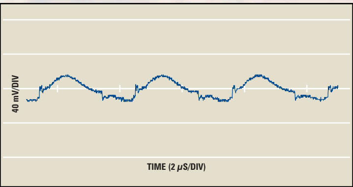
5V HDM+ RIPPLE
