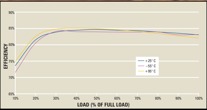
EFFICIENCY VS TEMPERATURE @ NOMINAL LINE 5V HDM+
